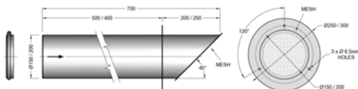
Horizontal Terminal 8 (can be cut to length)
