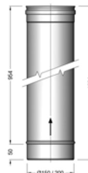
1000mm Straight
