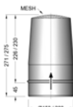
Top Stub (vertical discharge)
