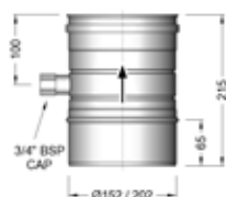
Flue Adaptor with Drain
