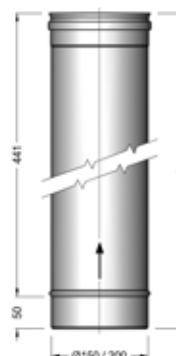
500mm Straight
