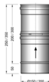
Adjustable Straight
