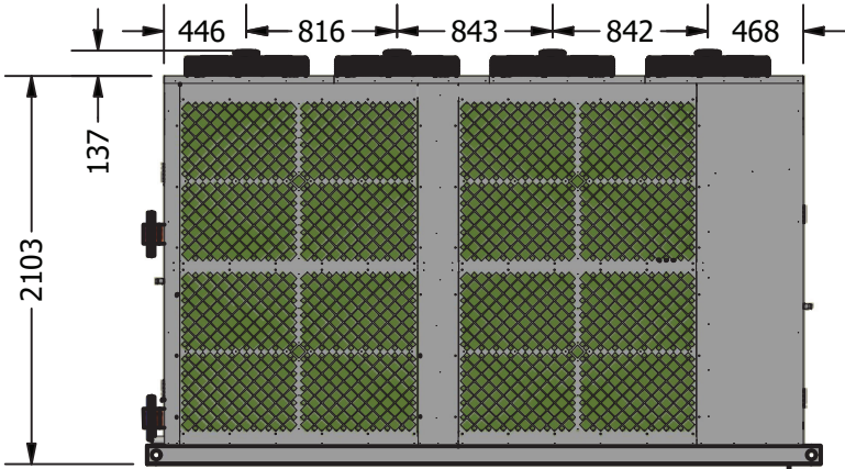
SIDE VIEW 3649
