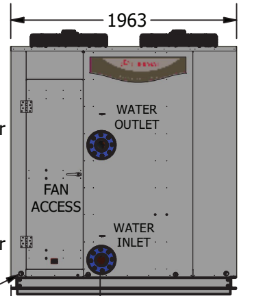
END VIEW
