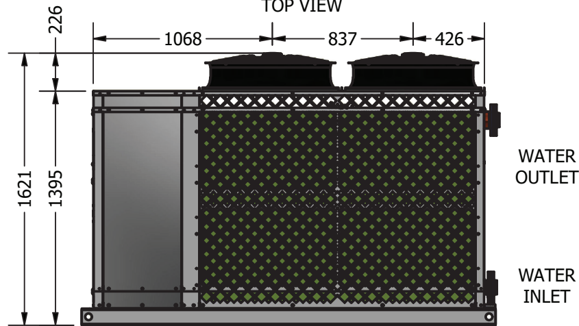
SIDE VIEW
