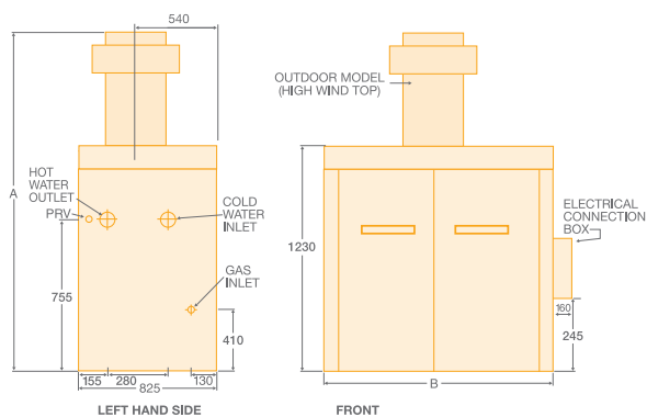
Models 972, 1142, 1242, 1362, 1662, 1852 (Outdoor)
