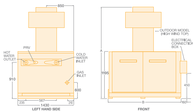
Models 2004, 2404, 2804 2 , 3304 2 , 3804 2 (Outdoor)
