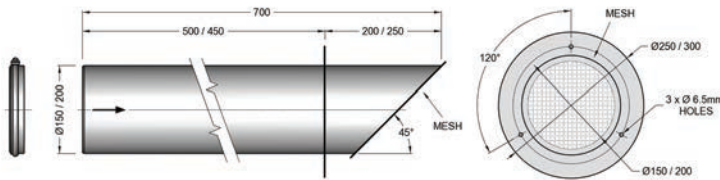
Horizontal Terminal ® (can be cut to length) Ø150mm - AQ94200121 Ø200mm - AQ94200144
