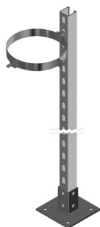
Outdoor Flue Stand Collar Ø150mm - AQ94200223 Ø200mm - AQ94200224 Base and Stand not included.
