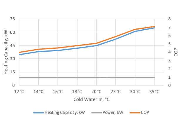
35 kW W2W COP and Heating Capacity
