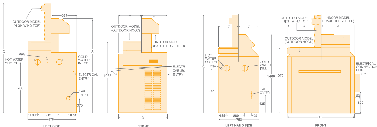
Models 200, 280, 350, 430 (Indoor/Outdoor)
