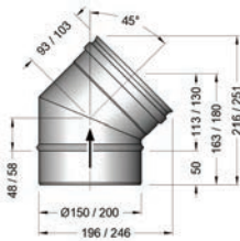
45° Elbow Ø150mm - AQ94200109 Ø200mm - AQ94200130
