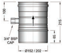
Flue Adaptor with Drain Ø150mm - AQ94200106 Ø200mm - AQ94200127
