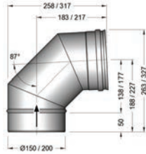
87° Elbow Ø150mm - AQ94200108 Ø200mm - AQ94200129
