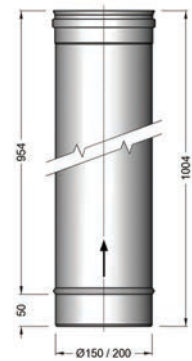
1000mm Straight Ø150mm - AQ94200110 Ø200mm - AQ94200131
