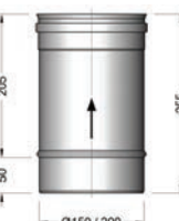
250mm Straight Ø150mm - AQ94200112 Ø200mm - AQ94200133
