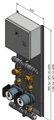
Standard Model
