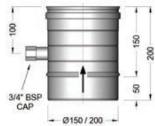
Flue Drain (project specific) Ø150mm - AQ94200107 Ø200mm - AQ94200128
