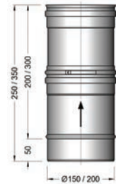
Adjustable Straight Ø150mm - AQ94200113 Ø200mm - AQ94200134
