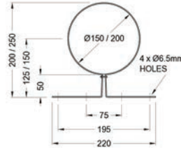
Mounting Band (1 per 1.5m of run) Ø150mm - AQ94200116 Ø200mm - AQ94200137
