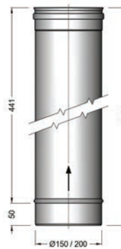
500mm Straight Ø150mm - AQ94200111 Ø200mm - AQ94200132
