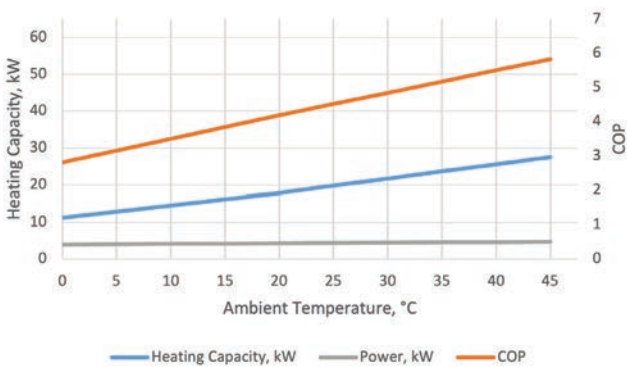
16 kW A2W COP and Heating Capacity
